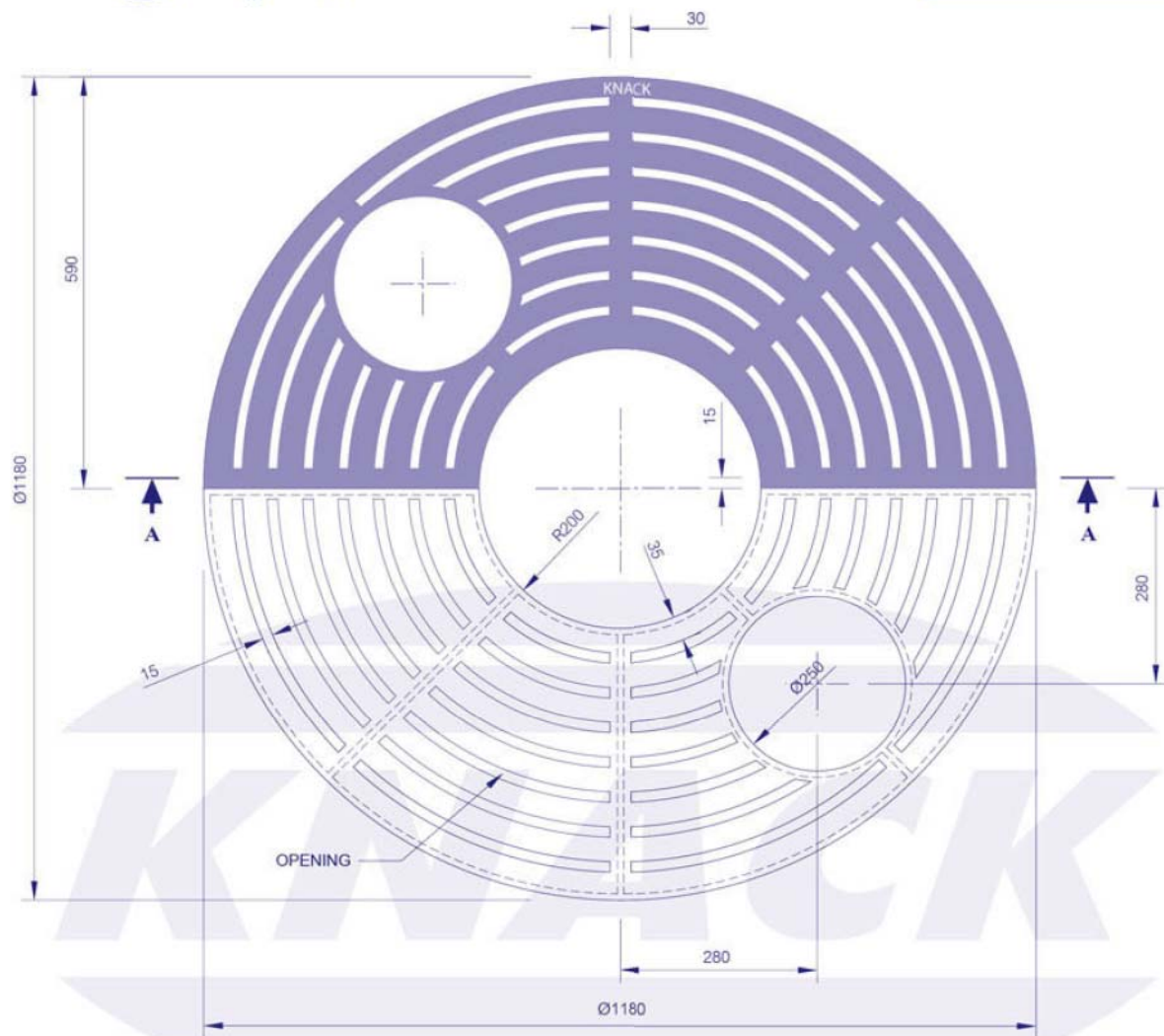
TOP VIEW
