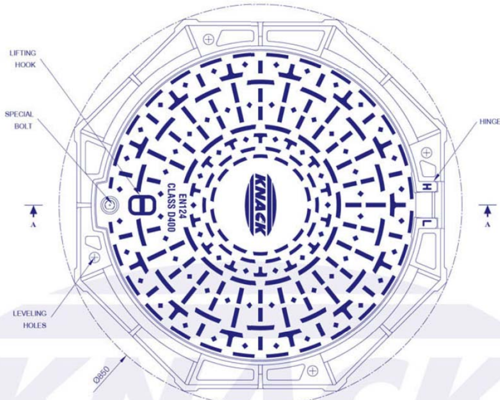
TOP VIEW
