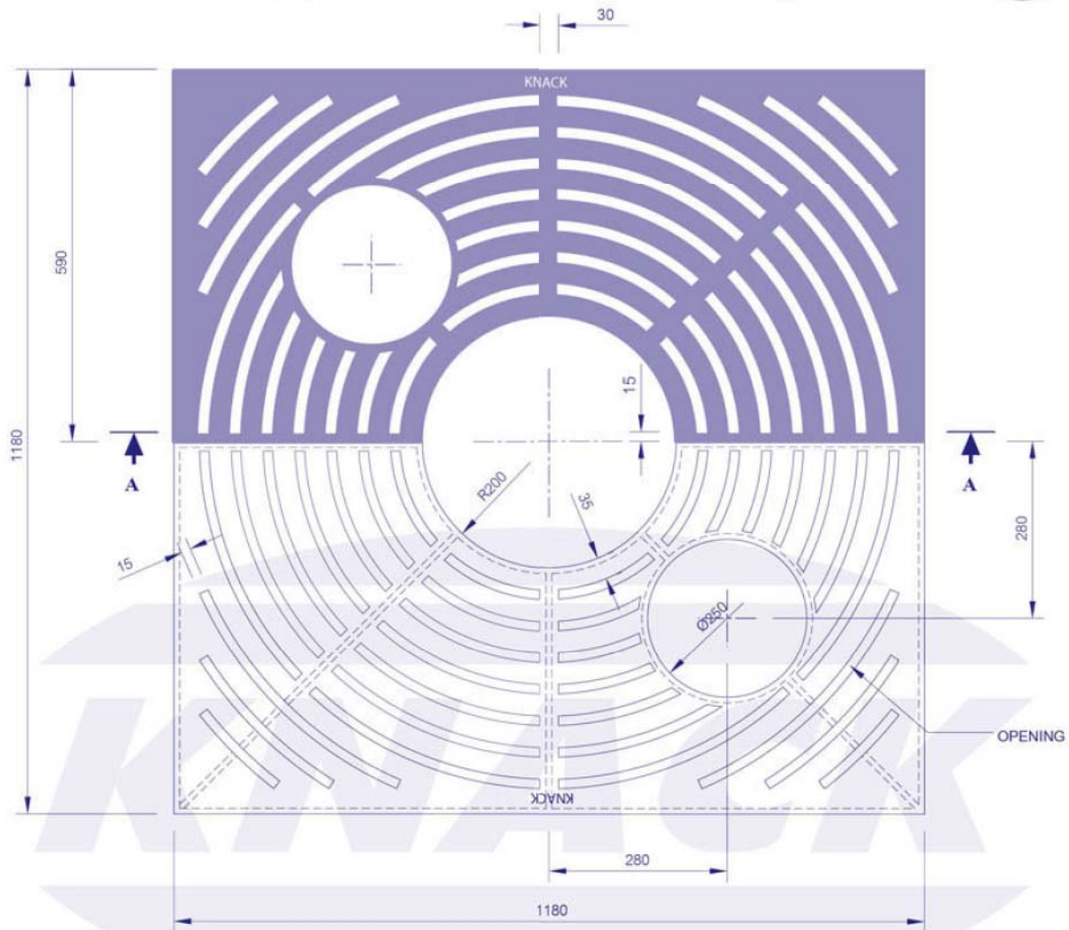
TOP VIEW
